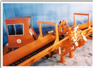
The trough-type infeed and outfeed conveyors are variable in length up to 80'.
