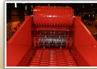
FEED SYSTEM Internal planetary drive with no chains and sprockets means lower maintenance, more torque and better durability.
