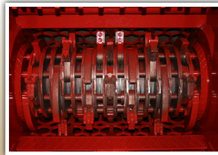
HAMMERMILL Laser-cut upturn rotor, factory balanced with forged hammers offer unsurpassed durability and smooth operation.
